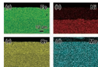
マグネシウム液体中に浸漬してニッケルが除去されたSUS316L表面層断面を示すEDS分析結果 EDS results on cross section of SUS316L surface in which toxic Ni element has been selectively removed in a Mg liquid
