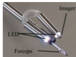
腹腔内手術用変形型内視鏡(外径5mm) Bending Transformative Endoscope for Intraoperative Surgery(O.D. 5mm)
