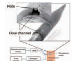
皮膚貼付型生体成分計測用微小流路付金属針と流路断面(針外径200 \mu m) Metal needle with micro flow channel for biological substances monitoring patch Cross-section view of flow channel (needle O.D. 200 \mu m).
