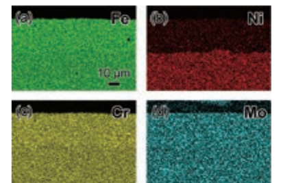
マグネシウム液体中に浸漬してニッケルが除去されたSUS316L表面断面を示すEDS分析結果 EDS results on cross section of SUS316L surface in which toxic Ni element has been selectively removed in a Mg liquid
