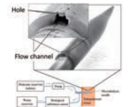
皮膚貼付型生体成分計測用微小流路付金属針と流路断面(針外径200μm) Metal needle with micro flow channel for biological substances monitoring patch Cross-section view of flow channel (needle O.D. 200μm).
