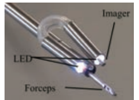
腹腔内手術用変形型内視鏡(外径5mm) Bending Transformative Endoscope for Intraoperative Surgery (O.D. 5mm)
