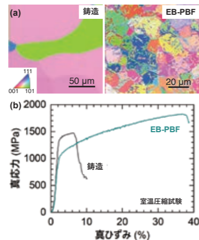
電子ビーム積層造形(EB-PBF)と鋳造を用いて作製した多成分系合金の(a)組織と(b)力学特性。合金組成は同じでも作製方法の違いを反映して異なる組織が得られ、力学特性に大きな影響を及ぼす。(a) Microstructures and (b) mechanical properties of a multi-principal element alloy prepared using electron beam powder bed fusion (EB-PBF) additive manufacturing and conventional casting. Despite having the same alloy composition, variations in manufacturing methods result in distinct microstructures, thereby exerting a significant impact on mechanical properties.
